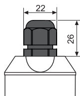
Variant "B" with standard cable gland
