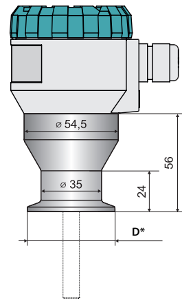
Tri- Clamp
