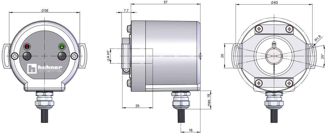
Drawing connection type 1, anti-rotation system type 3 (flexible flange 90.1027) and measuring range type CB0 or CBL
