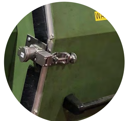
HD-11-C – with chain · Die-Cast or 316 Stainless Steel 316
