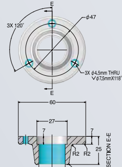
3/4" NPT ADAPTER TYPE
