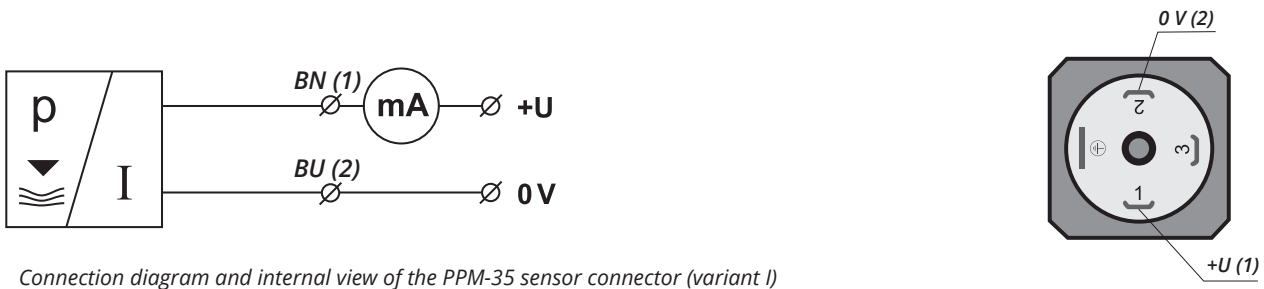
Connection diagram and internal view of the PPM-35 sensor connector (variant I)
