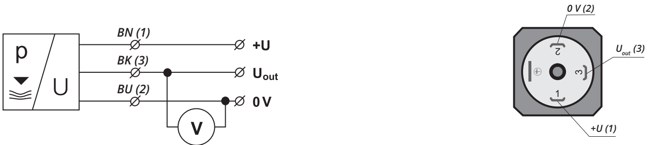
Connection diagram and internal view of the PPM-35 sensor connector (U variant)
